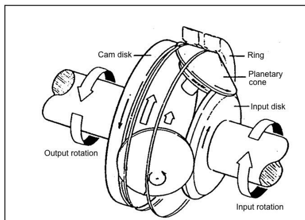
Rolling friction CVT
