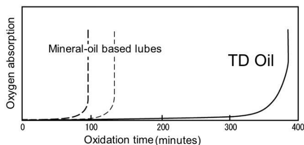
Oxidation stability (RPVOT)
