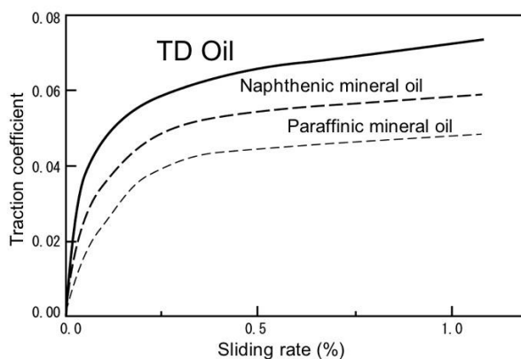
Traction characteristics
